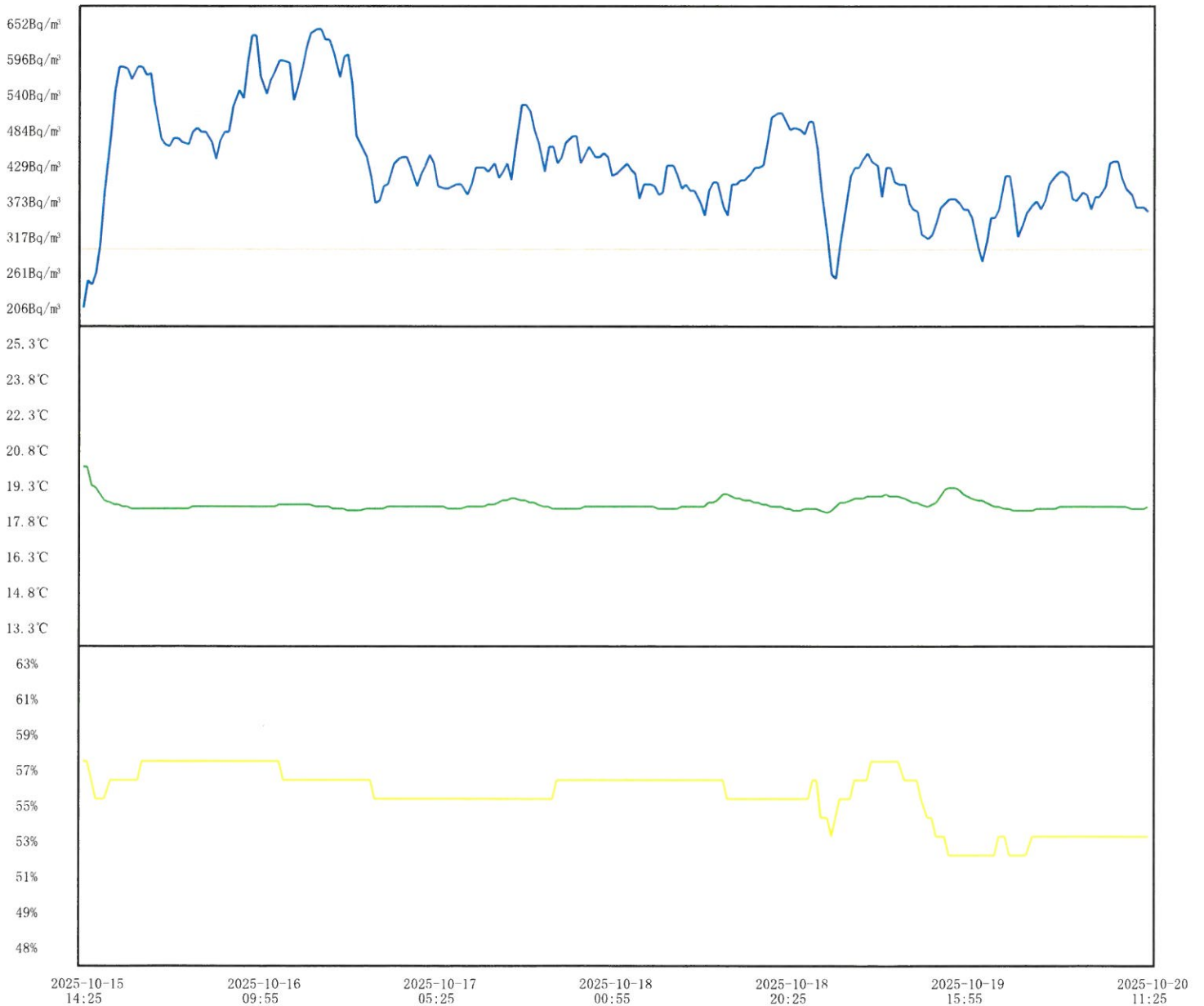
Historical details of radon concentration, temperature, and relative humidity (Red alert line:300Bq/m 3 )
